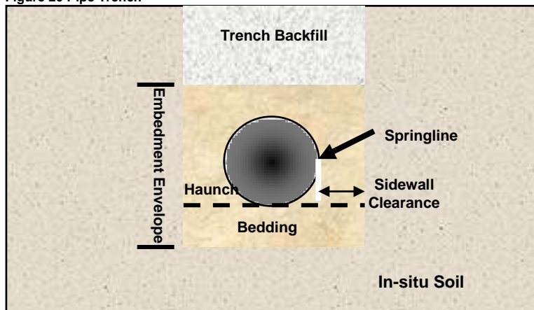
Figure 20 Pipe Trench
