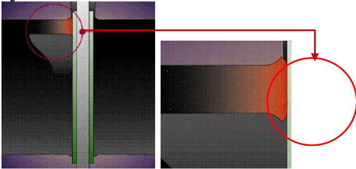
Figure 29: Butt Fusion Proper Bead Appearance
