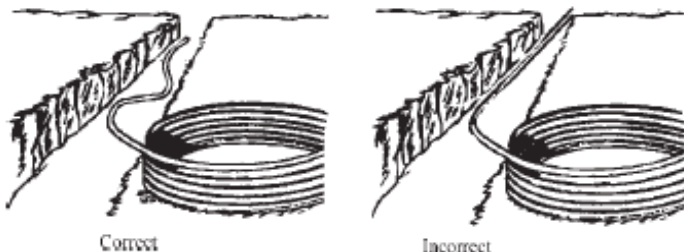
Figure 10: Proper vs. Improper Placement in Trench
