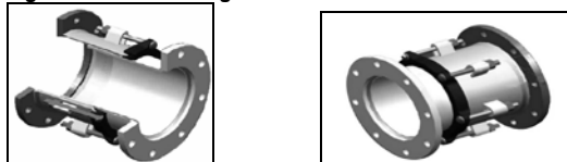
Figure 82: Dismantling Joint
