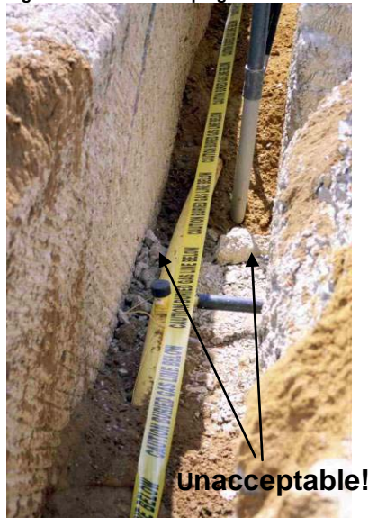
Fig. 25: Avoid Rock Impingement when Placing Embedment
