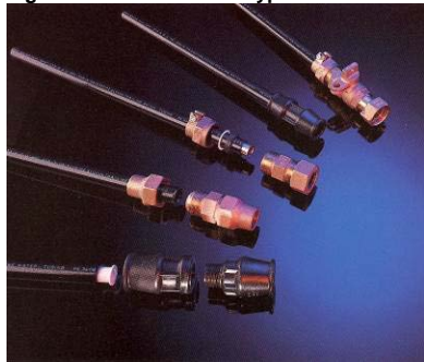
Figure 15 – HDPE Insert Type Mechanical Coupling
