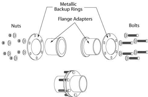
Figure 78 : Fange Connection Components
